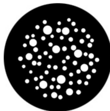
fixed gobo code: GOD00F-003 (Big Dots) Ø 31,5 mm image: Ø 23 mm pos. 6
