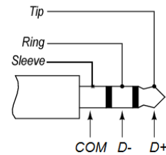
3.5mm TRS Plug
