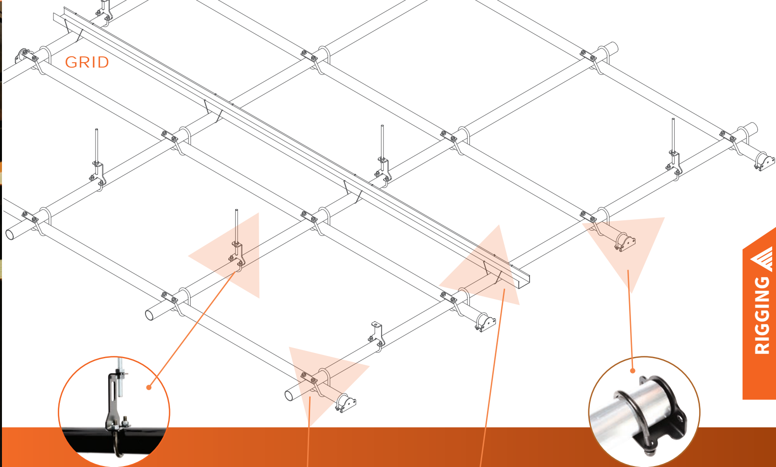
GRID BRACKETS adjustable in height
