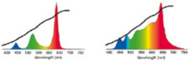
RGB(W) vs. 6-COLORS: AMBER, CYAN and LIME have been singled out as the perfect colors to complement the gaps in wavelength found in typical RGB systems.
